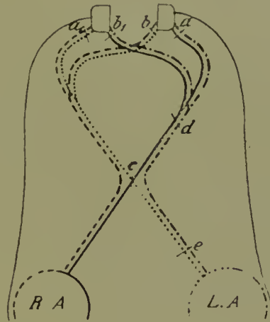
FIG. 38.—Diagram of relation of the optic tracts to the oculo-motor centres (Bumke). a , b , or a I , b I , position of lesion causing unilateral reflex iridoplegia, together causing double reflex iridoplegia; c , optic chiasma; d , position of lesion causing Wernicke's hemiopic reaction; e , optic nerve; R.A. , L.A. right and left eyeball respectively.
